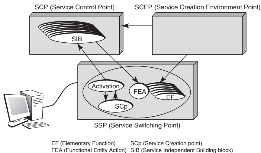
Figure W.9 Architecture IN/2
