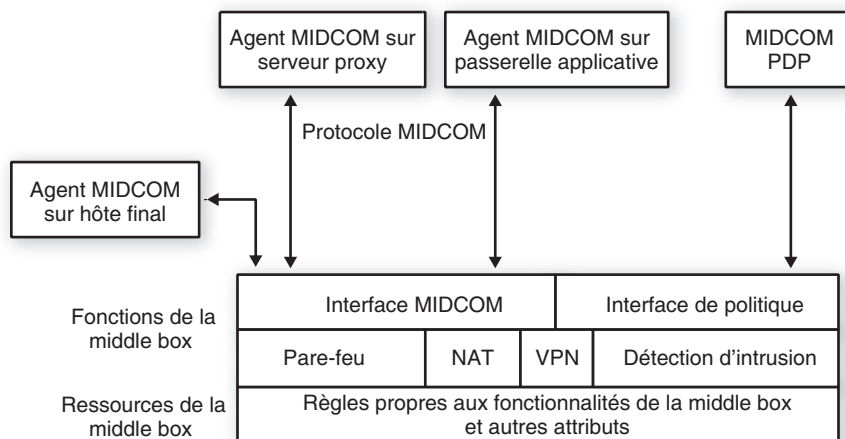
Figure T.12 Architecture d'une middle box
