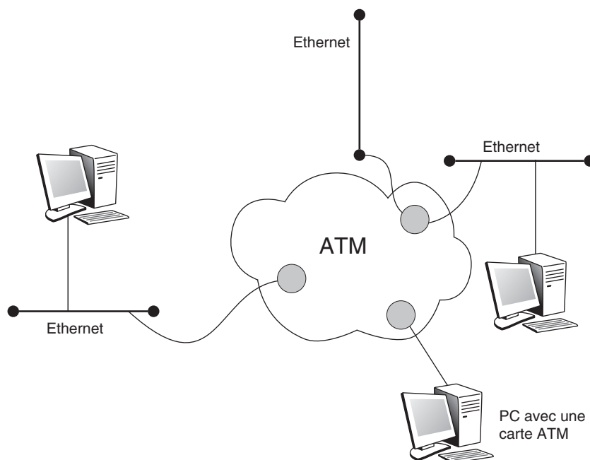
Figure L.2 Architecture LANE
