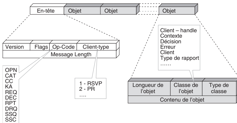
Figure S.19 Message COPS
