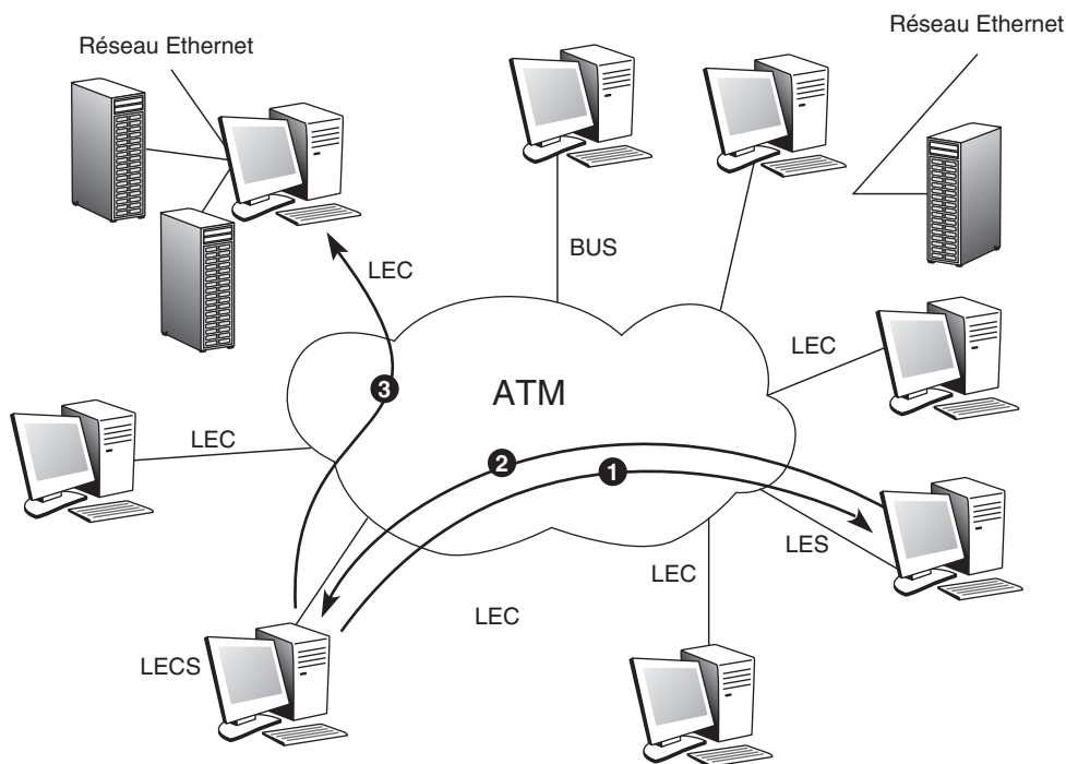
Figure L.3 Émulation L-UNI
